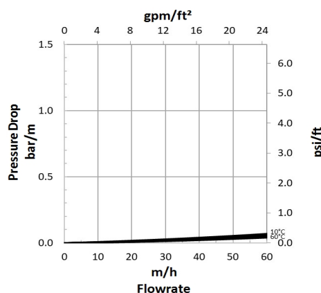
Figure 1a: Pressure Drop
