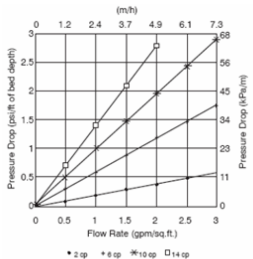
Figure 2: Pressure Drop
