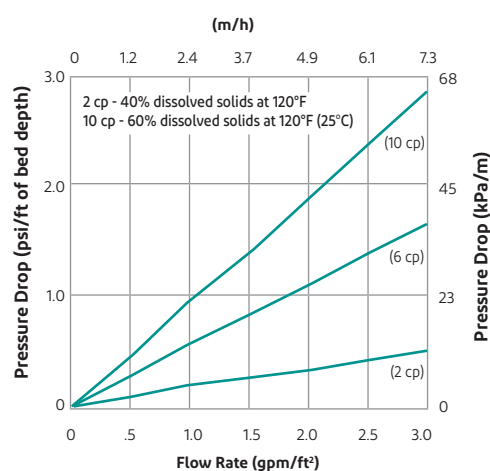
Figure 2. Pressure Drop Viscosity = 2 – 10 cP
