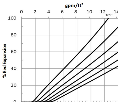
Figure 1: Backwash Expansion
