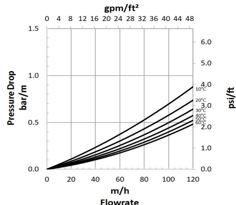
Figure 2: Pressure Drop
