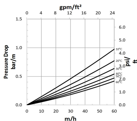
Figure 2: Pressure Drop
