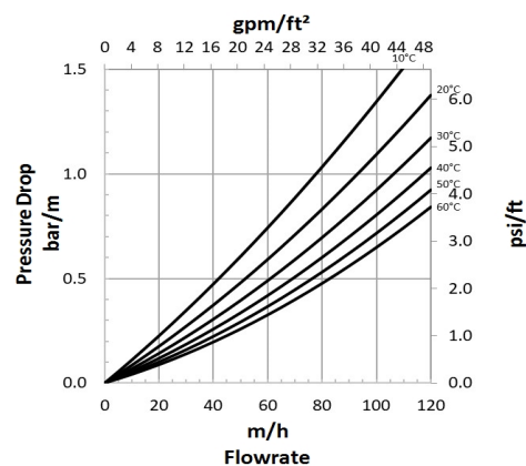
Figure 2: Pressure Drop
