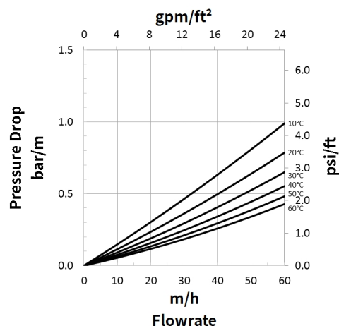
Figure 2: Pressure Drop
