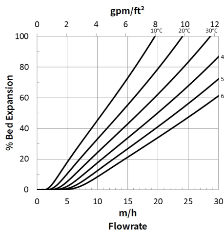
Figure 1: Backwash Expansion
