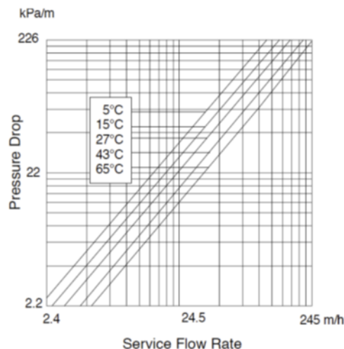
Figure 2: Pressure Drop
