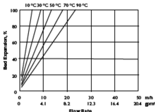
Figure 1: Backwash Expansion
