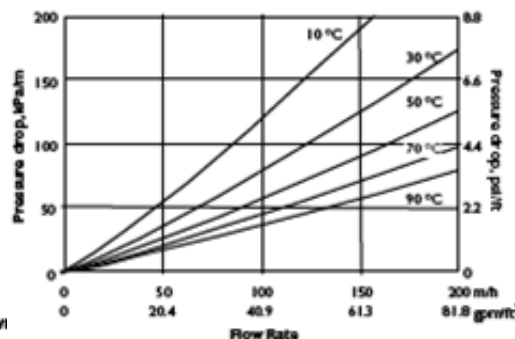
Figure 2: Pressure Drop
