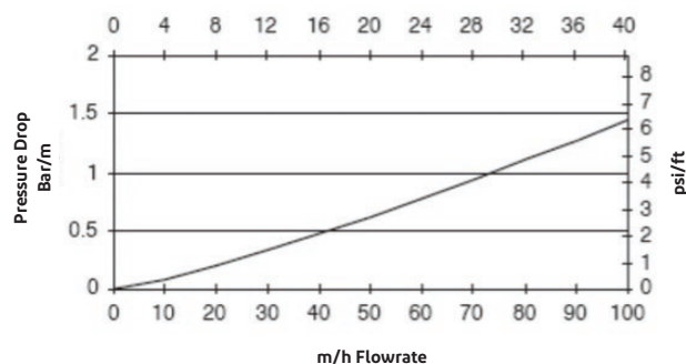
Figure 1. Pressure Drop Temperature = 20 °C (68 °F)
