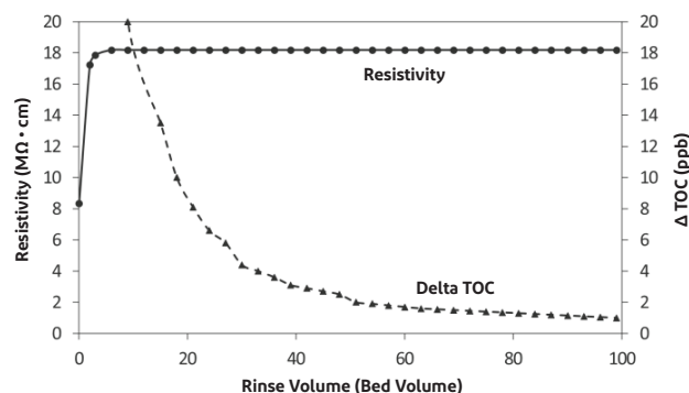
Figure 2: Resistivity and TOC Rinse Performance
