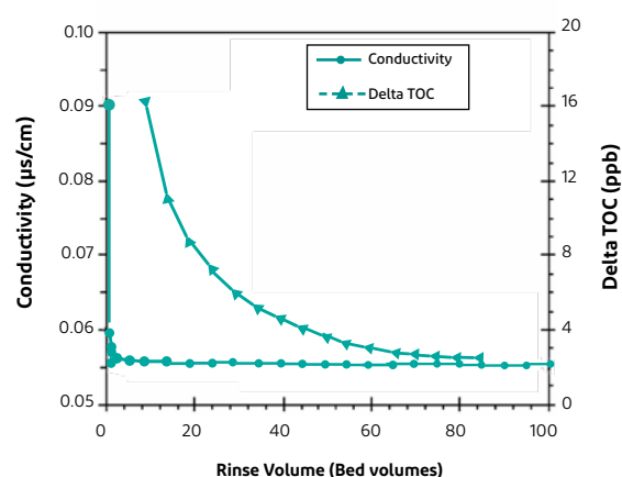
Figure 2: Resistivity and TOC Rinse Performance
