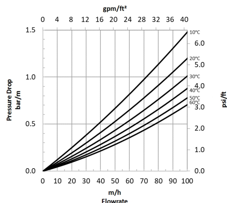
Figure 2: Pressure Drop
