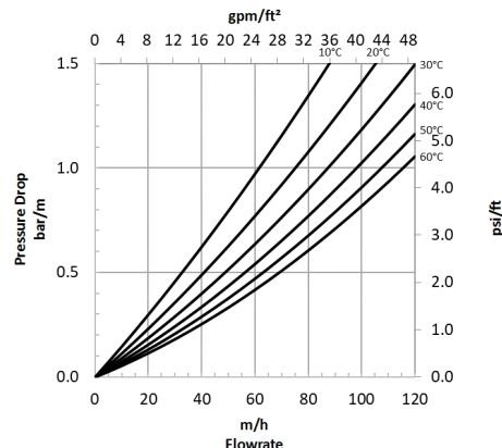
Figure 2: Pressure Drop
